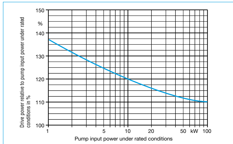
Fig. 20: Drive power as a function of rated pump input power at the operating point
